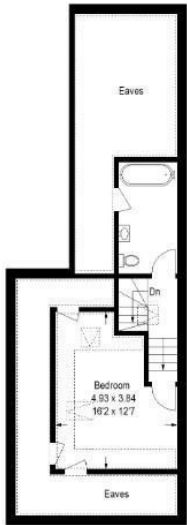
Second Floor
